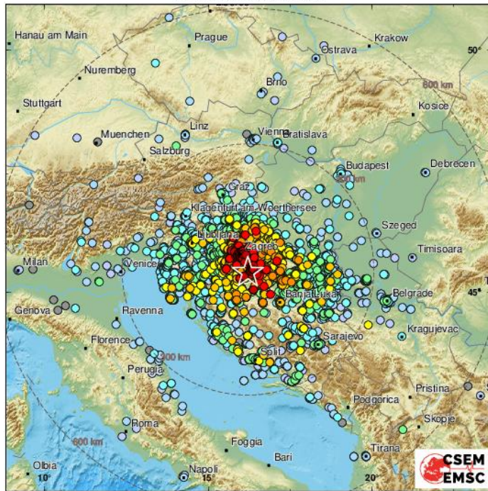
Felt reports received for M6.4 earthquake in CROATIA on 2020-12-29 11:19:54 UTC
